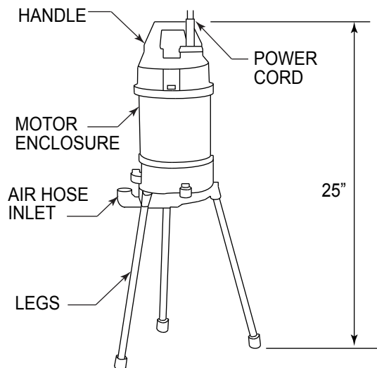
SIDE VIEW DIAGRAM
